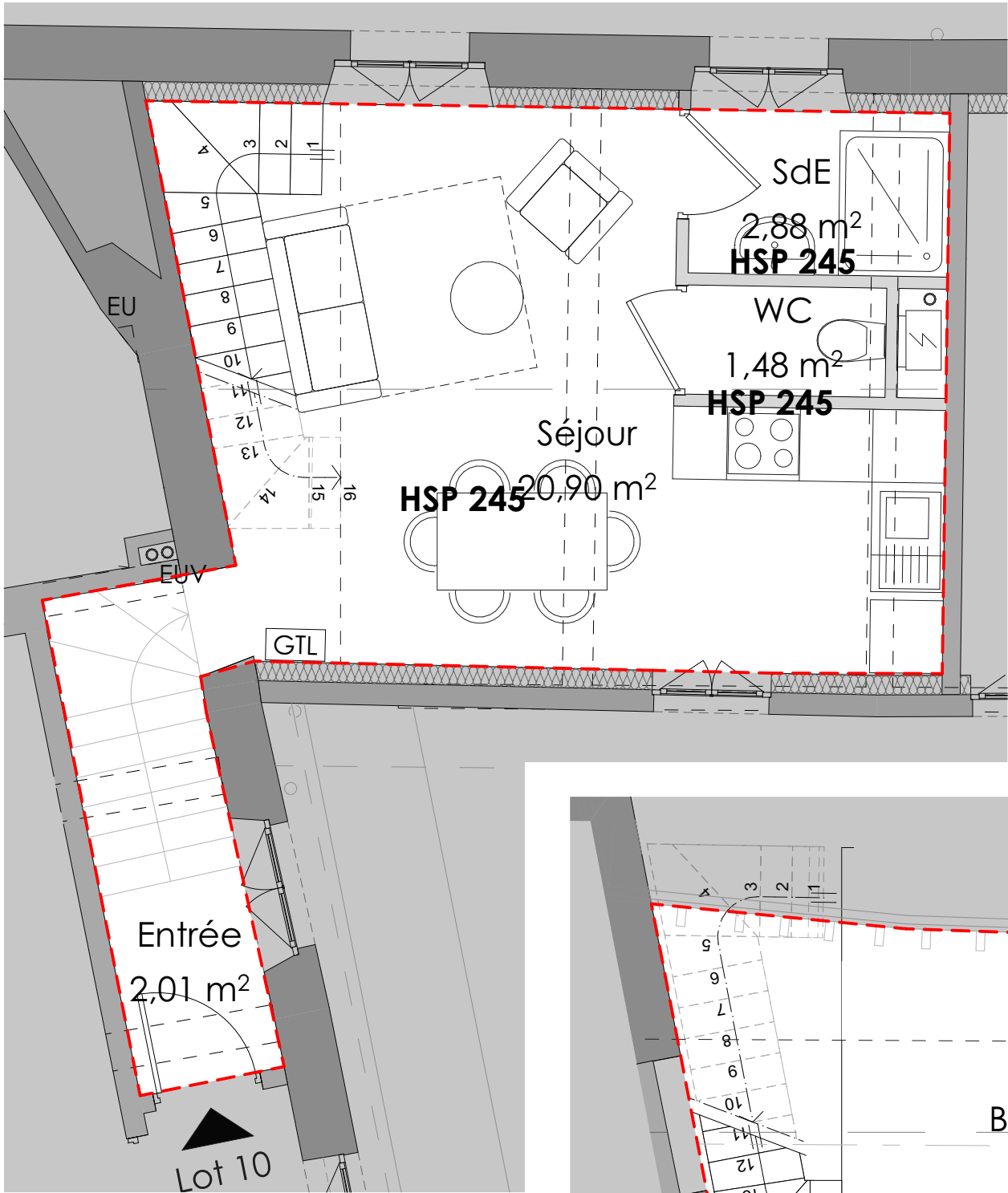
Plan R+1
