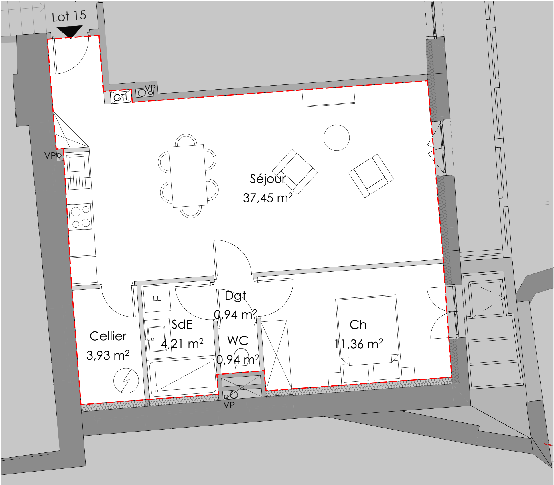
Plan R+1
